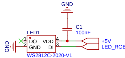
LED
