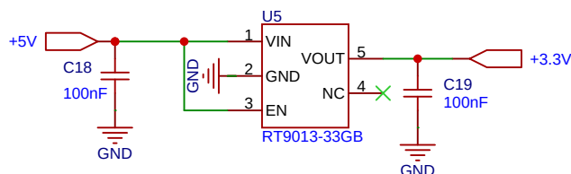
LDO - 3.3V
